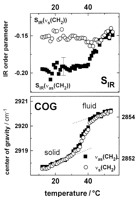
Fig. 4 Infrared order parameter ( S_{\text{IR}} ) and center of gravity (COG) of the antisymmetric (black squares) and symmetric (open circles) methylene stretching vibration of DTAB intercalated between ilerite layers at RH = 90% as a function of temperature. The left and right axes in the lower part correspond to \text{COG}(\nu_{\text{as}}(\text{CH}_2)) and \text{COG}(\nu_{\text{s}}(\text{CH}_2)) resp. In order to eliminate dichroic effects on the COG it was determined from the superposition of the polarized spectra A(\nu) = A_{\parallel}(\nu) + K_2 \cdot A_{\perp}(\nu) . The representative error bar corresponds to the standard error of five independent preparations
